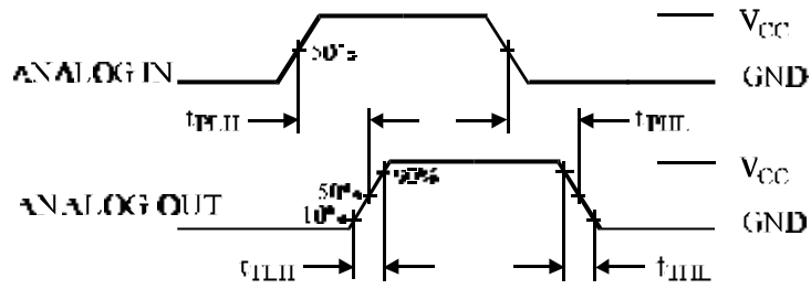
Figure 1. Switching Waveforms
